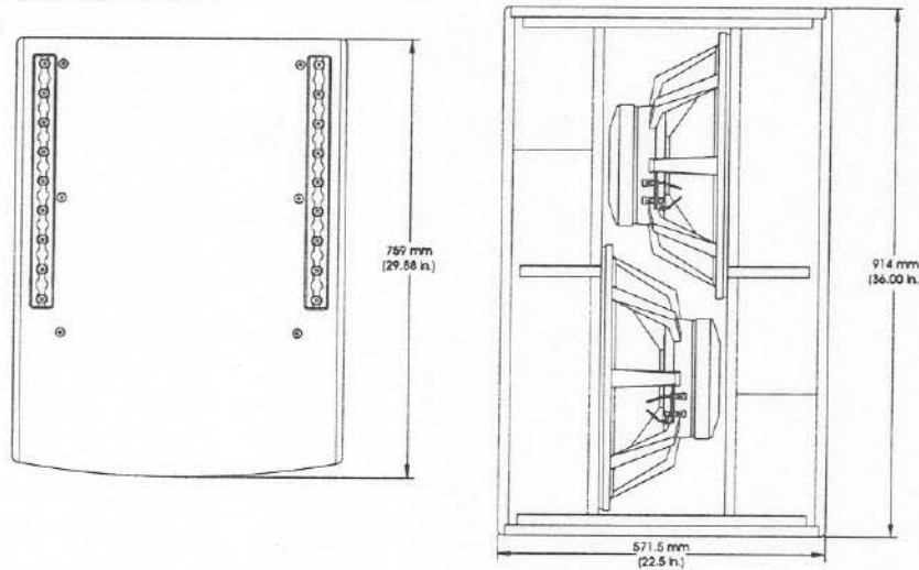
Figure 8—Dimensions
